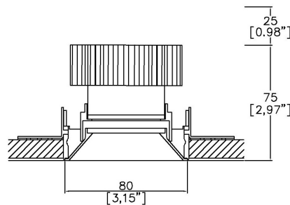
750+LED-TL/PCZ Cut-out 82mm Ø Trimless Kit
