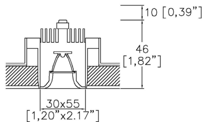
A2602-FL-TL Cut out 59 x 35mm (2.32" x 1.38")
