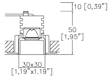
AM40-SS-TL Cut-out 41 x 41mm (1.61" x 1.61")
