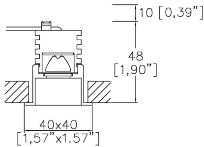
AM40-SS-TR Cut-out 37 x 37mm (1.46" x 1.46")
