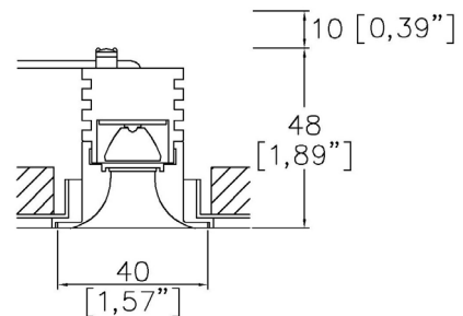
AM40-FL-TR Cut-out 37mm (1.46") Ø
