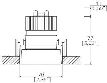
Soft70 Gen2 with Trimless Kit TL3 (1) (rear fitting, solid ceiling) Cut-out Ø70mm (Ø2,75"). Required depth height +15mm.
