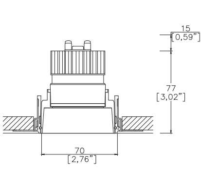
Soft70 Gen2 with Trimless Kit TL1 (1) (front fitting, full skim) Cut-out Ø83mm (Ø3,26"). Required depth height +15mm.
