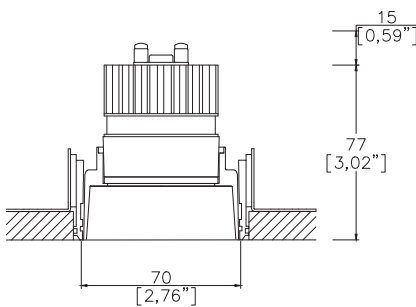
Soft70 Gen2 with Trimless Kit TL2 (1) (rear fitting, partial skim) Cut-out Ø82mm (Ø3,22"). Required depth height +15mm.
