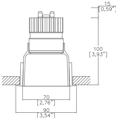
SF70100-TR1 (1) Cut-out Ø82mm (Ø3,22”). Required depth height + 15mm ^
