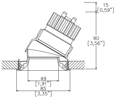
Mix85 Flare with Trim Kit TR1 (1) Cut-out Ø80mm. Required depth height+25mm.
