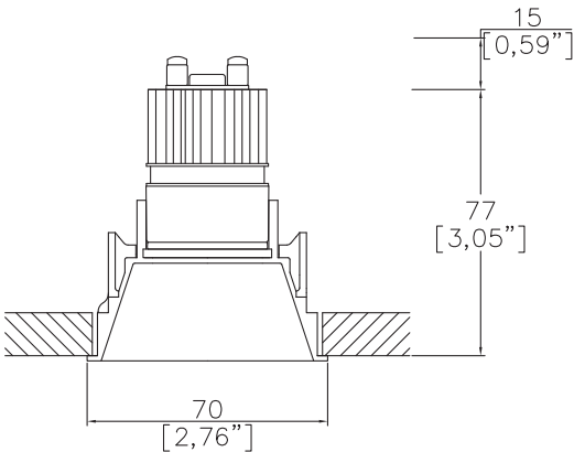
MT70200-TR1 Cut out Ø65mm Required depth height + 15mm^
