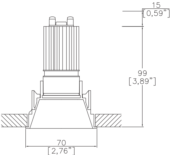
MT70200-TR1 Cut out Ø65mm Required depth height + 15mm^
