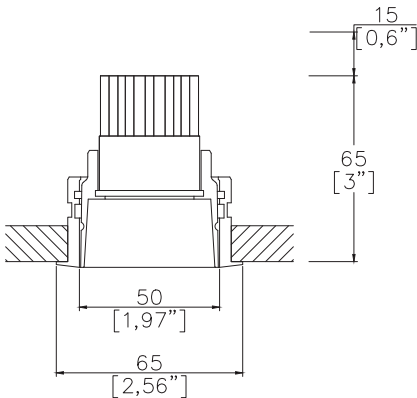
Soft50 Gen2 with Trim Kit TR1 (1) Cut-out Ø61mm. Required depth height +15mm.
