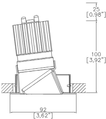
91413-WW-LED + 9000-PBZ Cut-out 83mm Ø Trim kit
