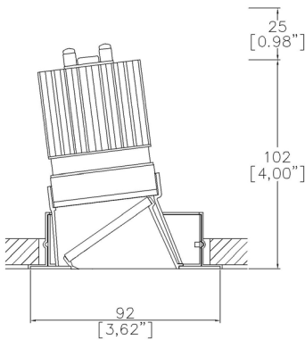
91413-WW-LED + 9000-PCZ Cut-out 83mm Ø Seamless flush appearance
