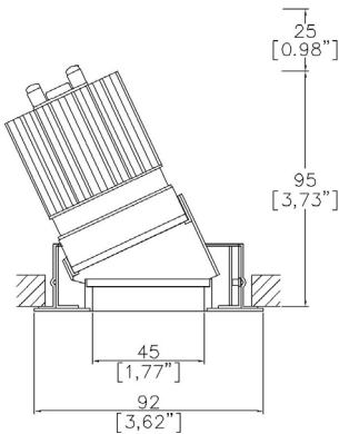
91413-A-LED + 9000-PBZ Cut-out Ø83mm Trim kit Required depth height+25mm^
