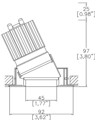
91413-A-LED + 9000-PCZ Cut-out Ø83mm Seamless flush appearance Required depth height+25mm^
