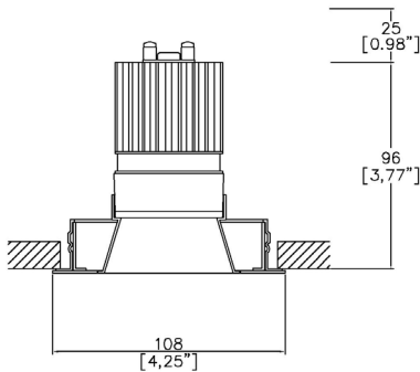
A31600-LED + 3000-PBZ Cut-out 103mm (4.00”) Ø
