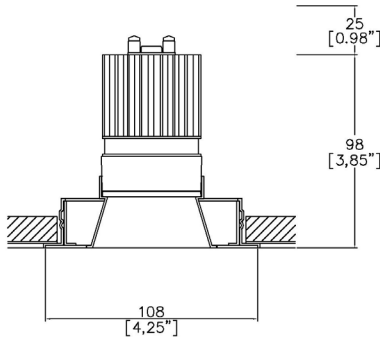
A31600-LED + 3000-PCZ Cut-out 98mm (3.85”) Ø
