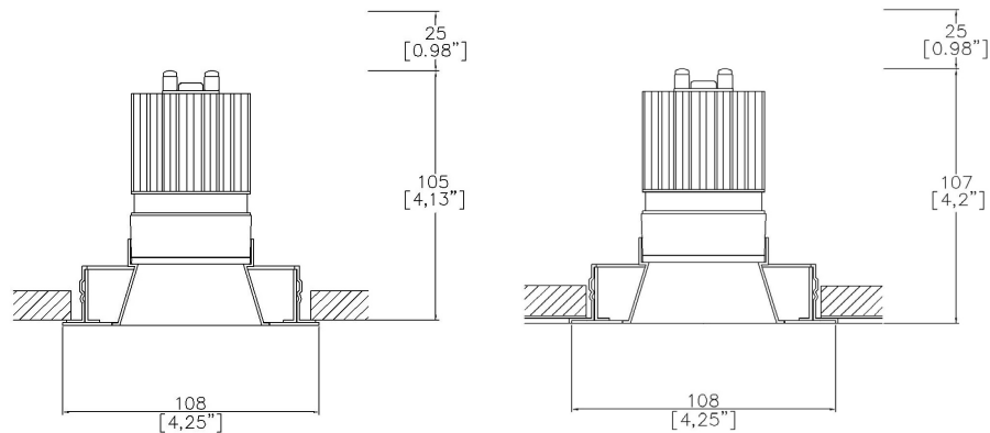
930-FL-LED + 9000-PBZ Cut-out 83mm Ø
