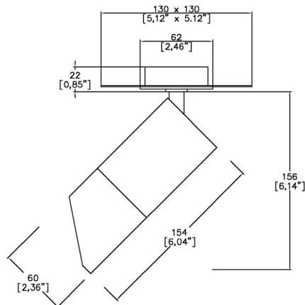
7100/2-LED-WW-TMP Cut out Ø57mm
