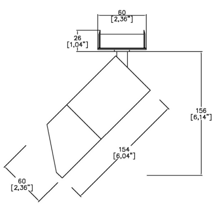
7100/2-LED-WW-RMP Cut out Ø57mm
