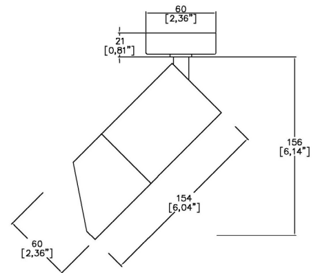
7100/2-LED-WW-SMP Cut out Ø15mm
